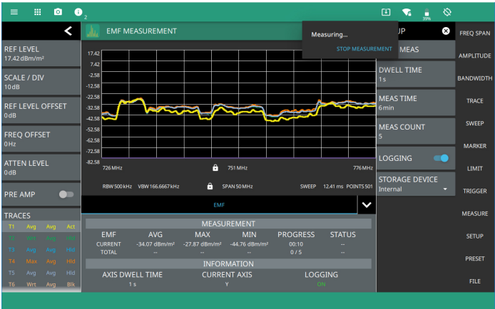
EMF Results Show Power from each Antenna Axis and Summary Results for Peak and Average Power over a Defined Time Period
