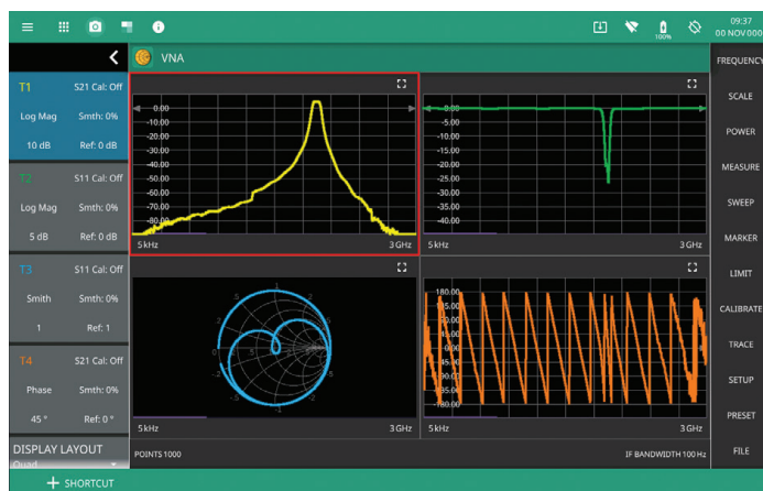
Quad Display Highlighting Essential Characteristics of a Bandpass Filter
