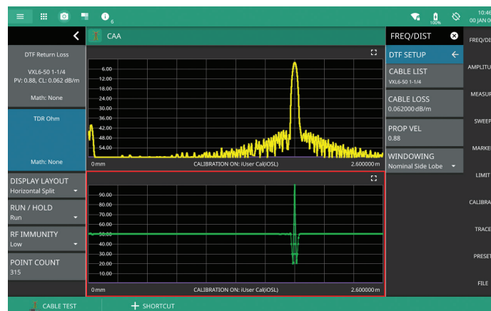
Split Screen Showing DTF and TDR Measurements
