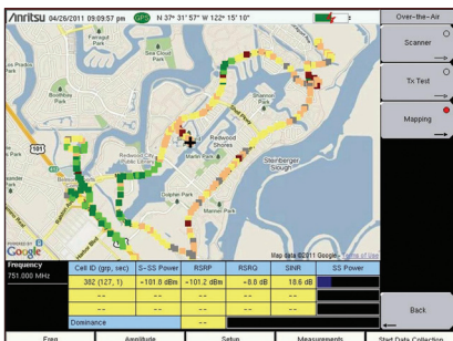
Over-the-Air On-screen Mapping With easyMap Tools™ Import Map Area on Instrument Screen to Drive Test Downlink Coverage of S-SS Power, RSRP, RSRQ, or SINR.
