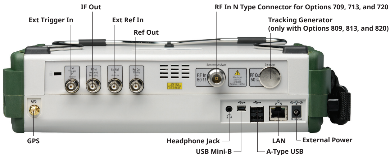
Connector Panel for MS2720T
