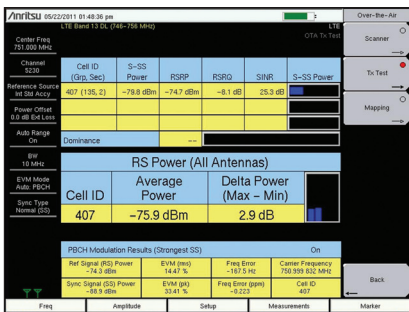
Over-the-Air Measurements – Tx Test By Looking at the Reference Signals of MIMO Antennas One Can Determine if MIMO is Working Properly. If the Delta Power is Too Large, There is an Issue.
