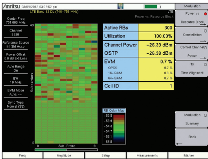
Modulation Quality – Power vs. Resource Block A High Utilization of the Resource Blocks Would Indicate a Cell Site in Nearing Overload and it May be Appropriate to Start Planning for Additional Capacity.
