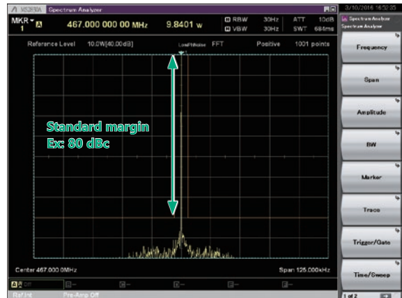
Spurious Emissions (out-of-band) Measurement Example
