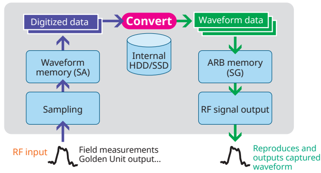
Playback Block Diagram
